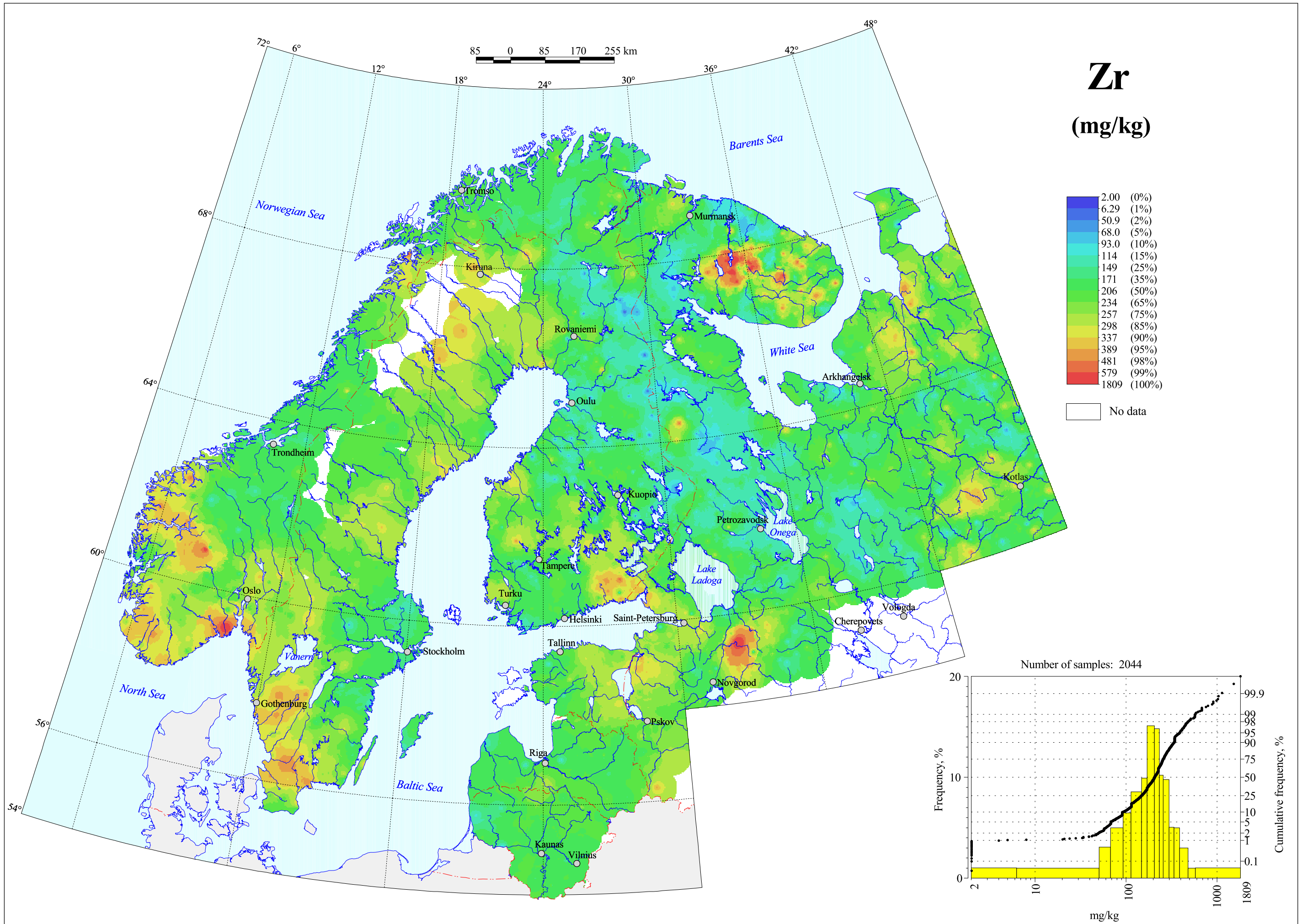
Zirconium in C-horizon, grain size <2mm, total content
